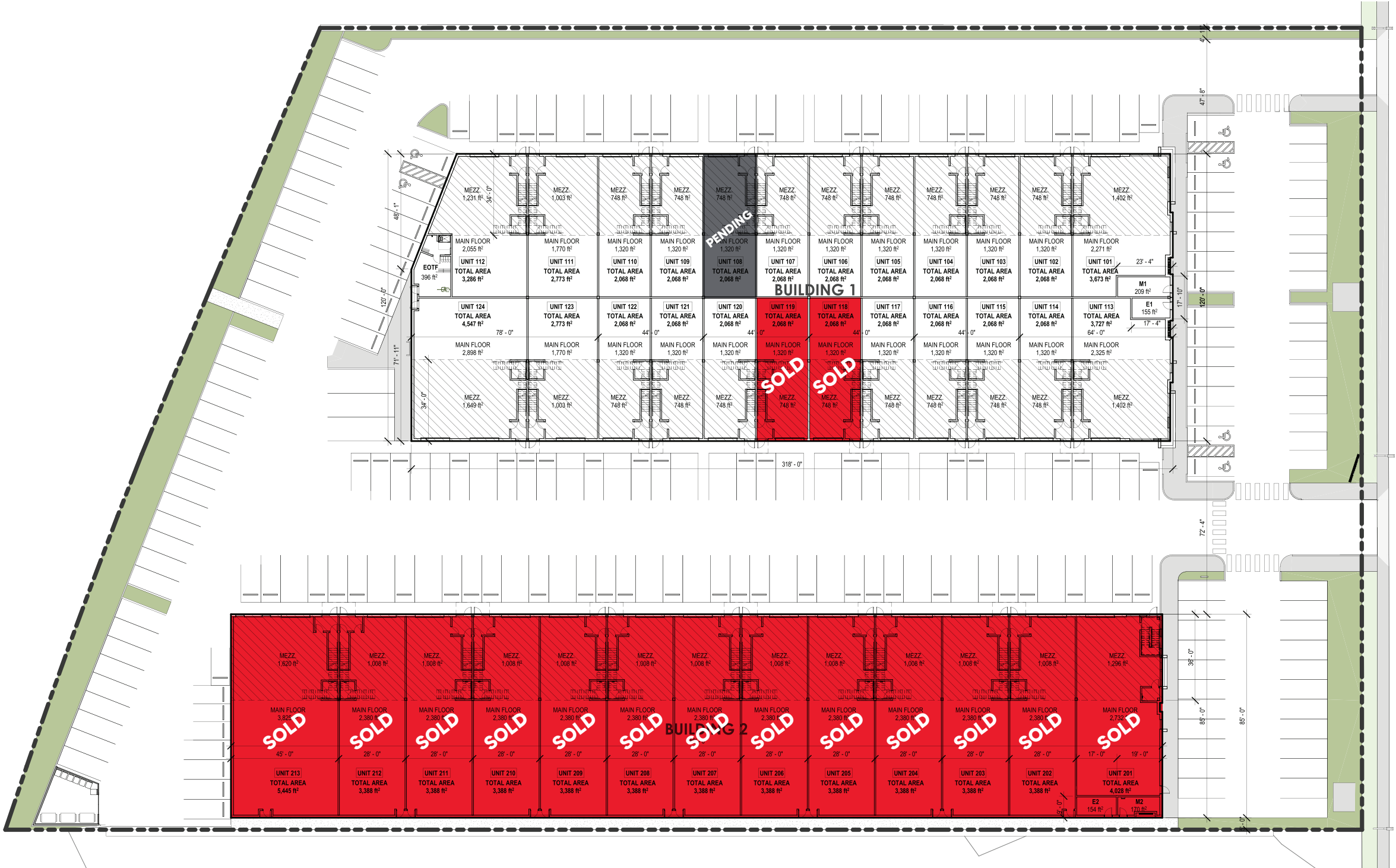
1 OVERALL SITE PLAN 3/64" = 1'-0"
